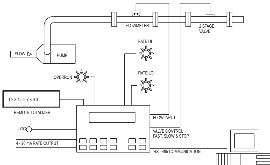
FIG. 4 - TYPICAL APPLICATION - BATCH / RATE CONTROL
