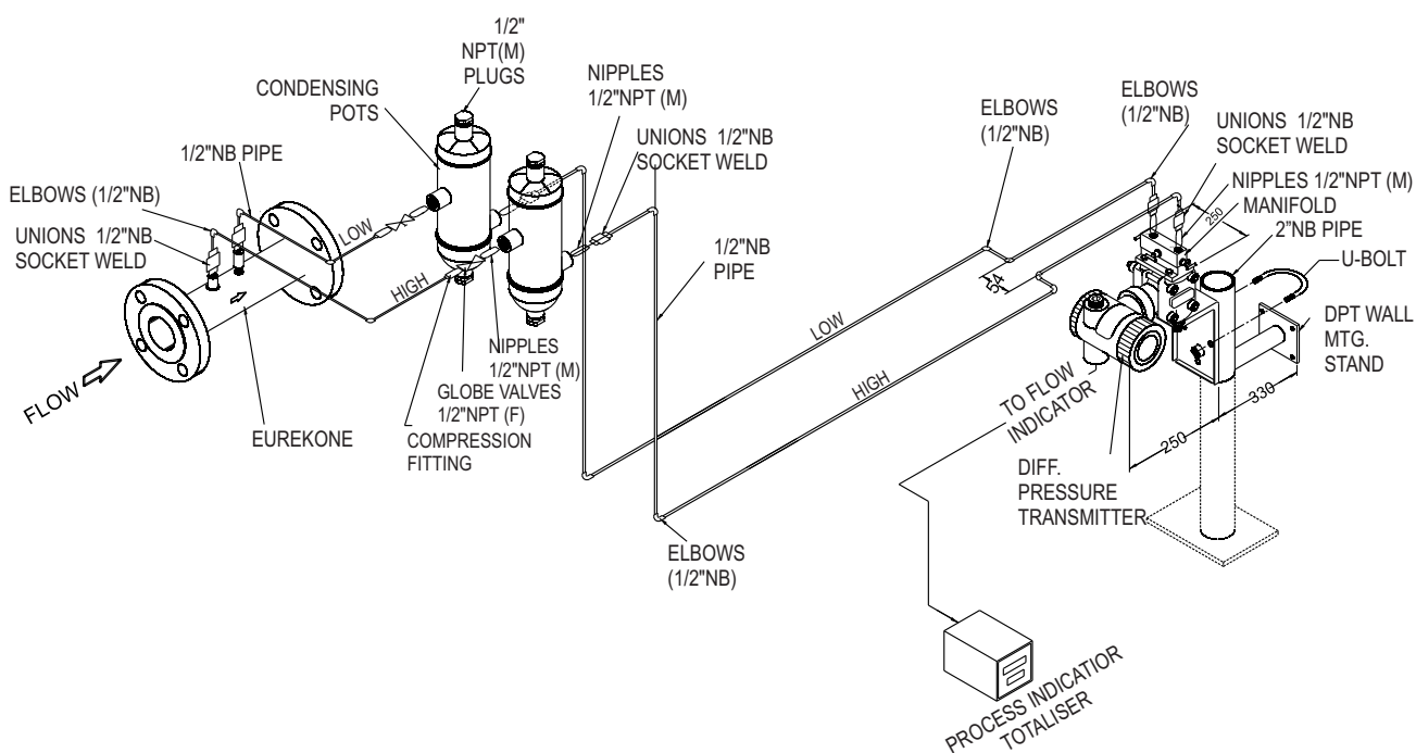
TYPICAL INSTALLATION DRG. STEAM APPLICATION ( WITH OR WITHOUT IBR )
